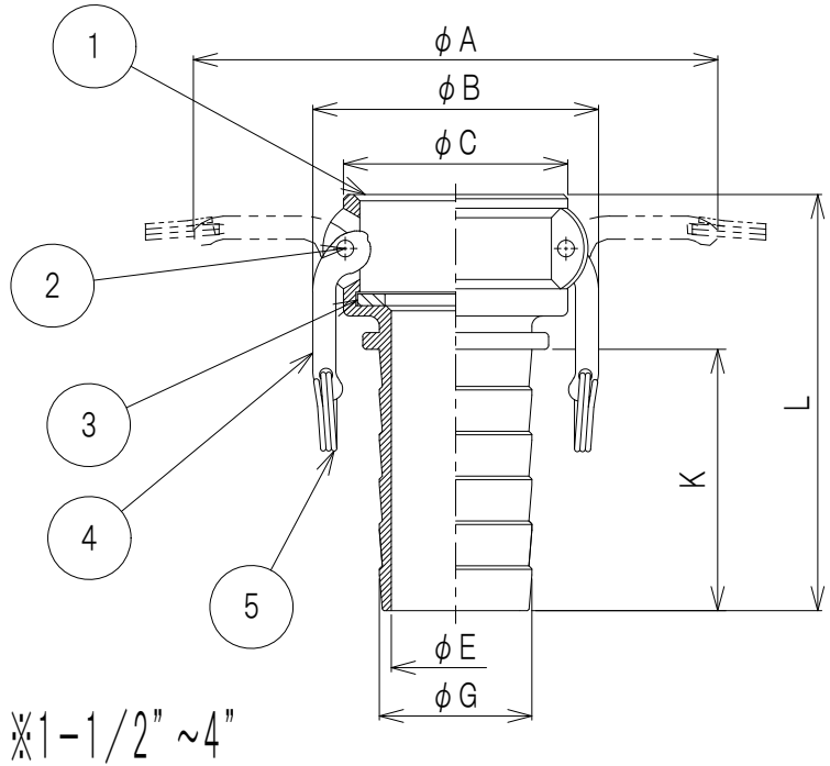
6 3 3 - C T S S T DIMENSION TABLE BY SIZES (UNIT:mm)
